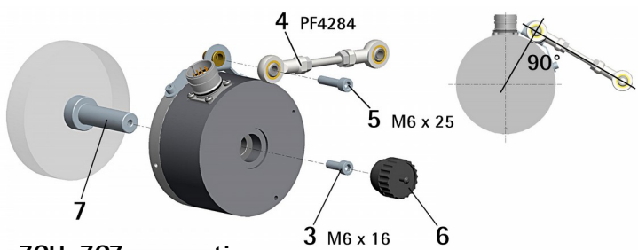
ZCU, ZCZ connections
